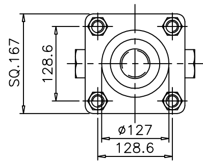
VIEW FROM ARROW A-A
